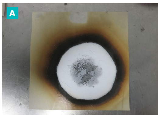
Figure 20: UP-laminate (15 wt.-% GF) after torch test: A) 300 phr APYRAL® HC 500 and B) 200 phr ACTILOX® HTB .
