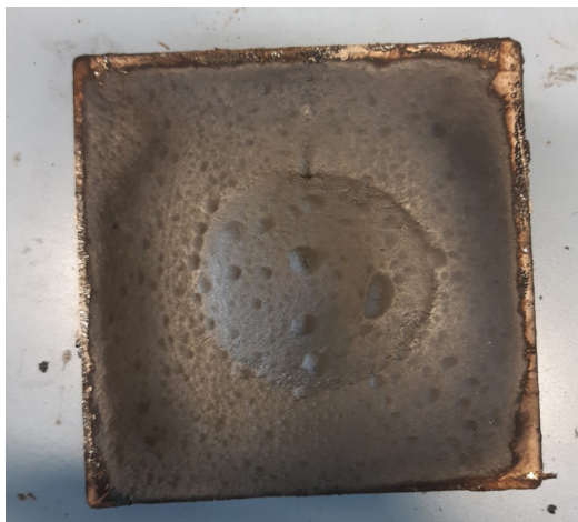
PA6_20%GF_40% ACTILOX® HTB -b No burn through within 20 min; very solid, ceramic like residue; backside temperature < 400 °C
