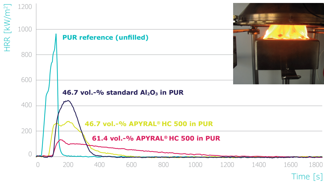
Figure 16: Cone measurement of PUR. Heat release rate of unfilled PUR in comparison with APYRAL® HC 500 and standard \text{Al}_2\text{O}_3 filled PUR.
