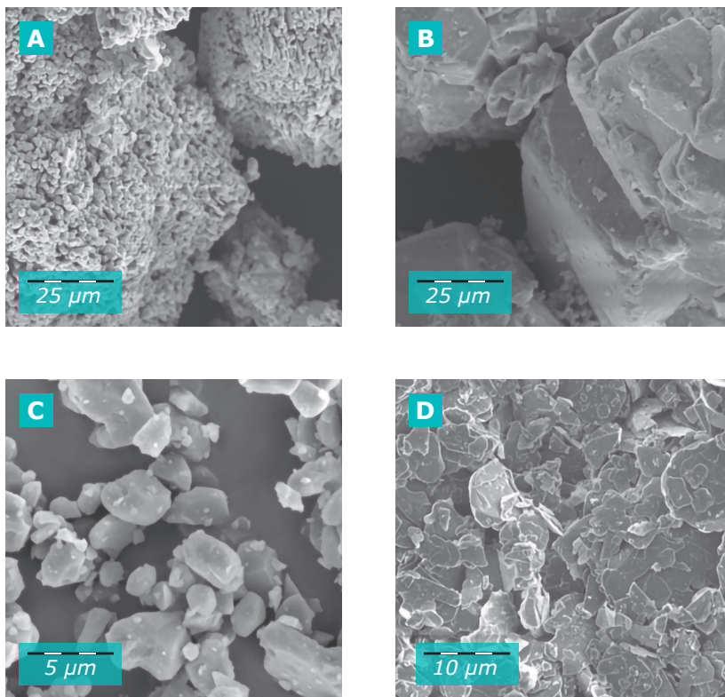
Figure 10: SEM-images of calcined alumina (80 \mu\text{m} , A), APYRAL® HC 500 (B), calcined alumina (3 \mu\text{m} , C), and BN (9 \mu\text{m} , D).
